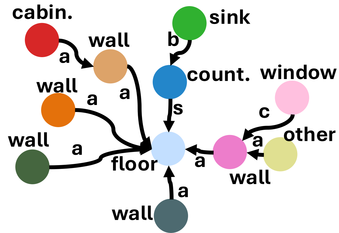
GT
